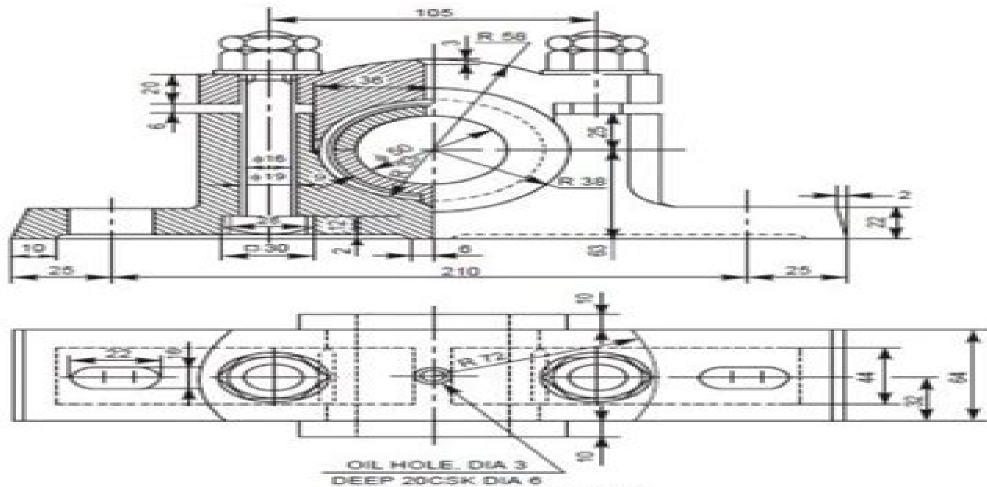
Fig. 12.4 Plummer block
