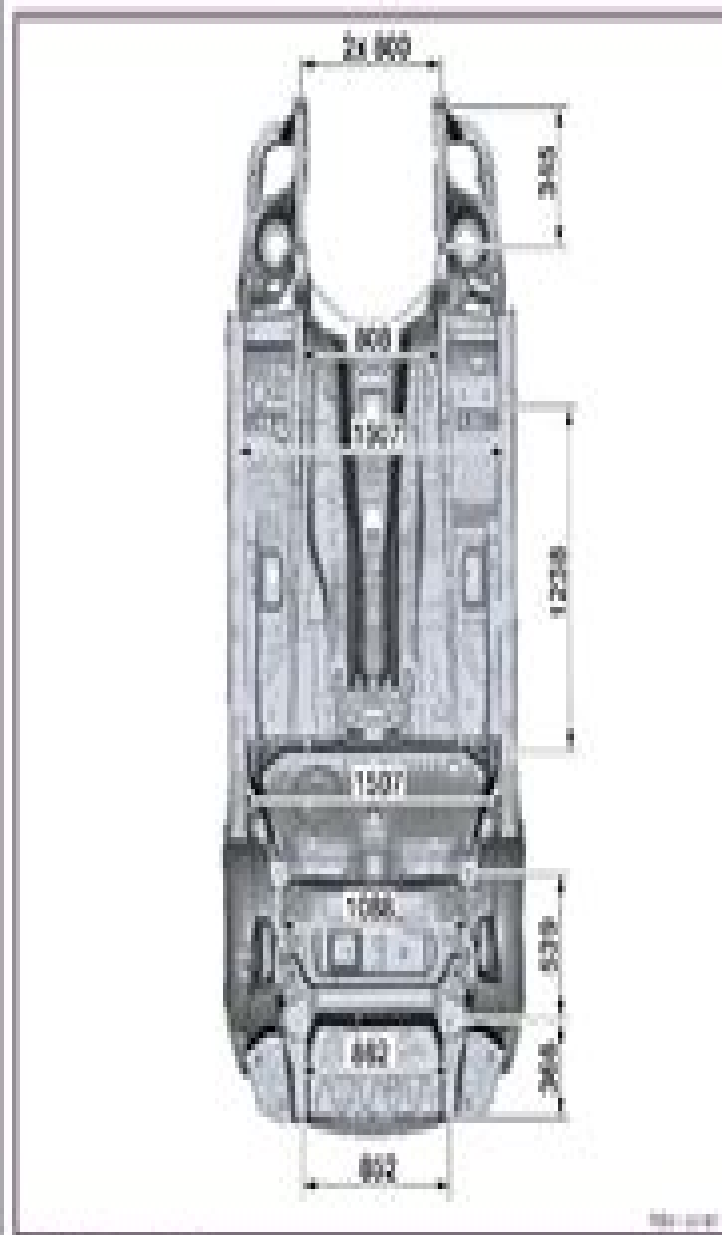
Underbody view 2
