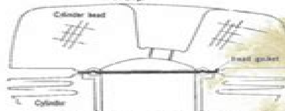
Fig. 6-1-2 Installing cylinder head gasket
