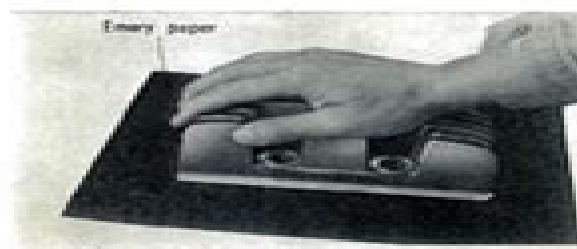
Fig. 6-1-1 Repairing cylinder head warp
