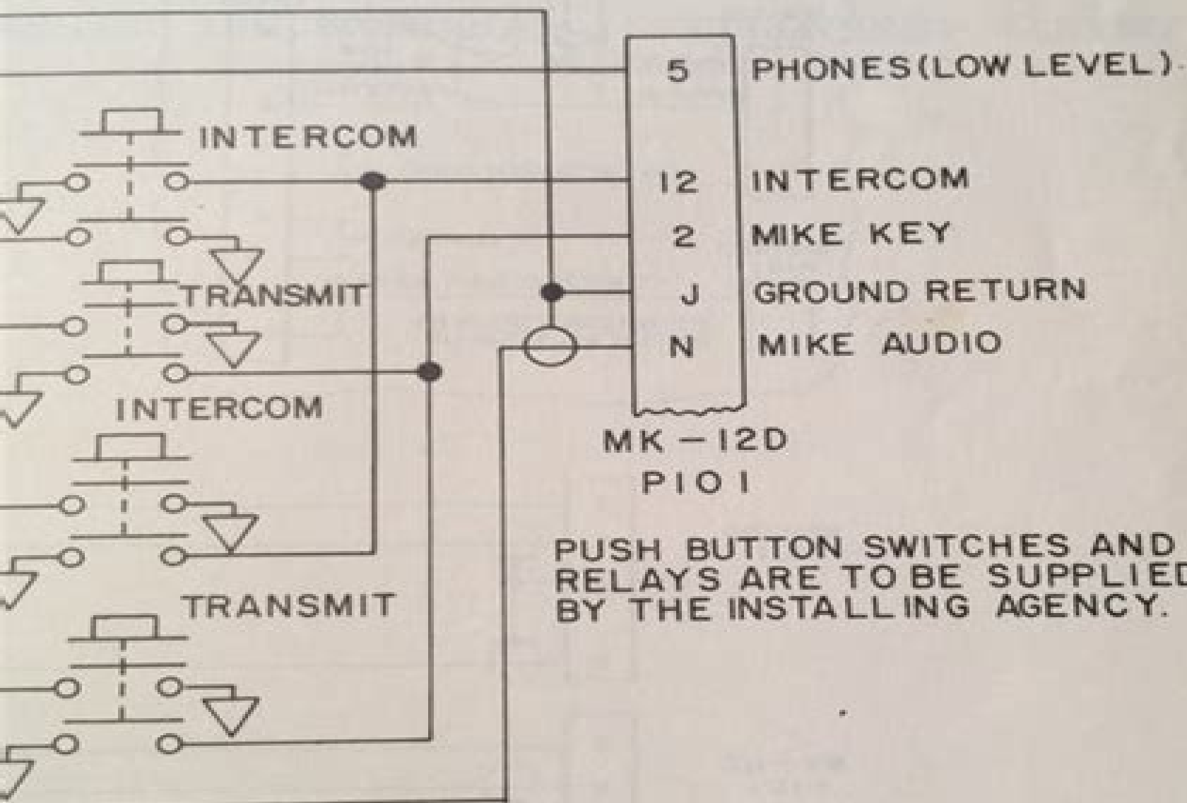
AIRCRAFT INTERCOM WIRING.
