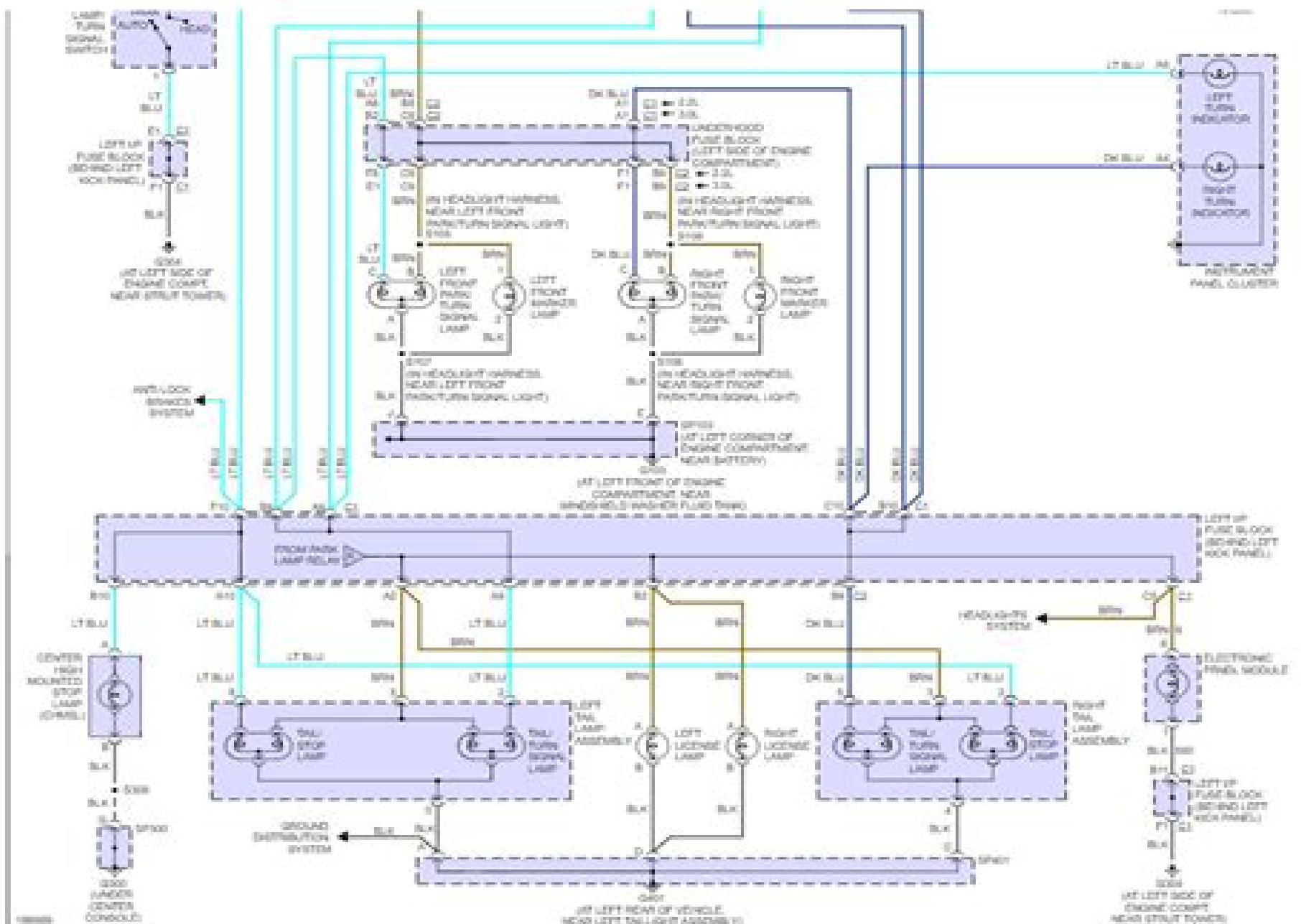
Fig 2: Exterior Lamps Circuit, Sedan
