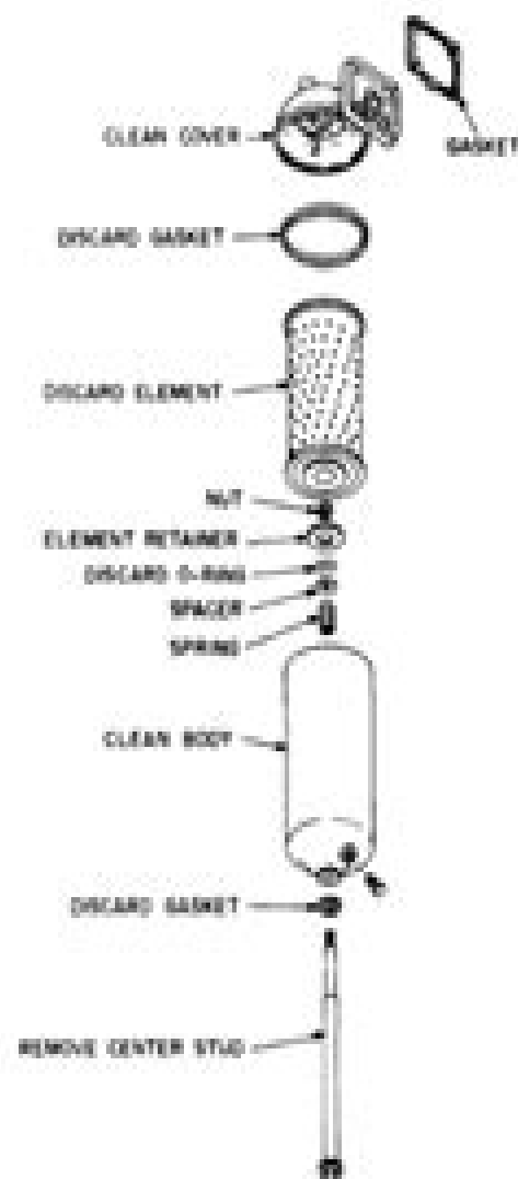
Figure 4-2. Oil filter service.
