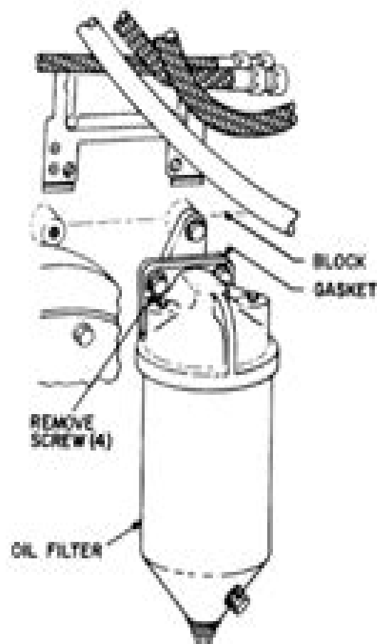
Figure 4-1. Oil filter, removal and installation.
