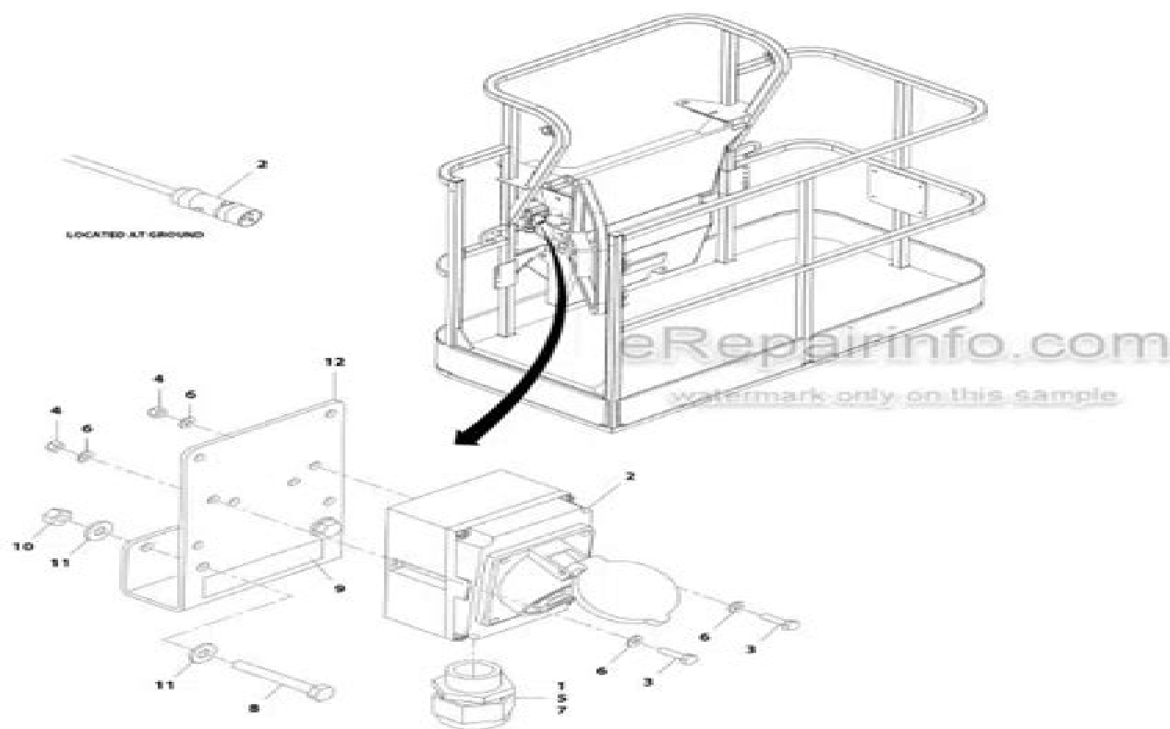
FIGURE 8-2. AC BOX AT PLATFORM - 110V IEC YELLOW (CE SPEC)
