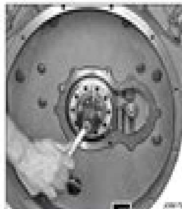
Figure 412 Crankshaft seal removed (stripped chassis)
