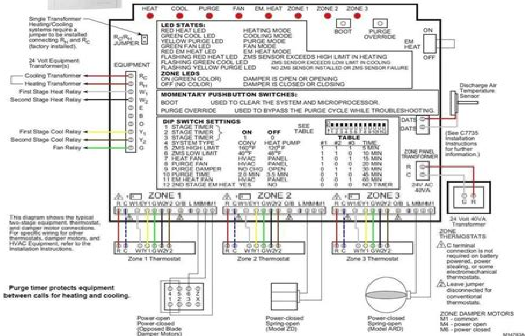
Fig. 13. EMM-3U System wiring diagram.
