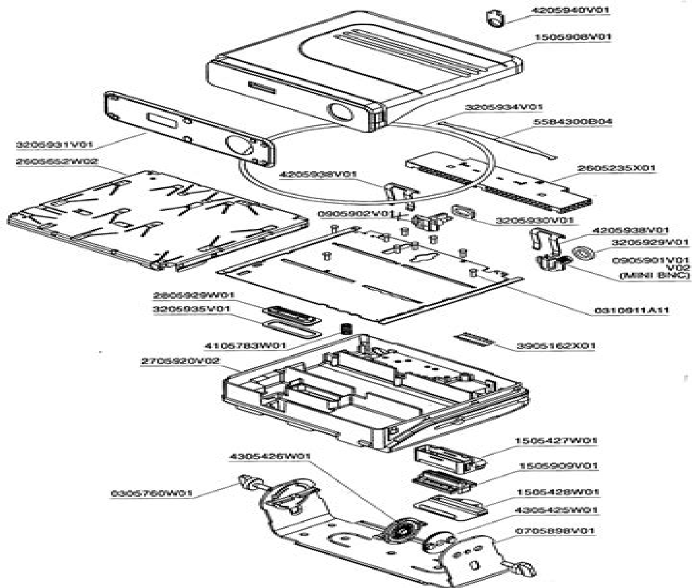
TRANSCEIVER EXPLODED VIEW DIAGRAM AND PART NUMBERS
