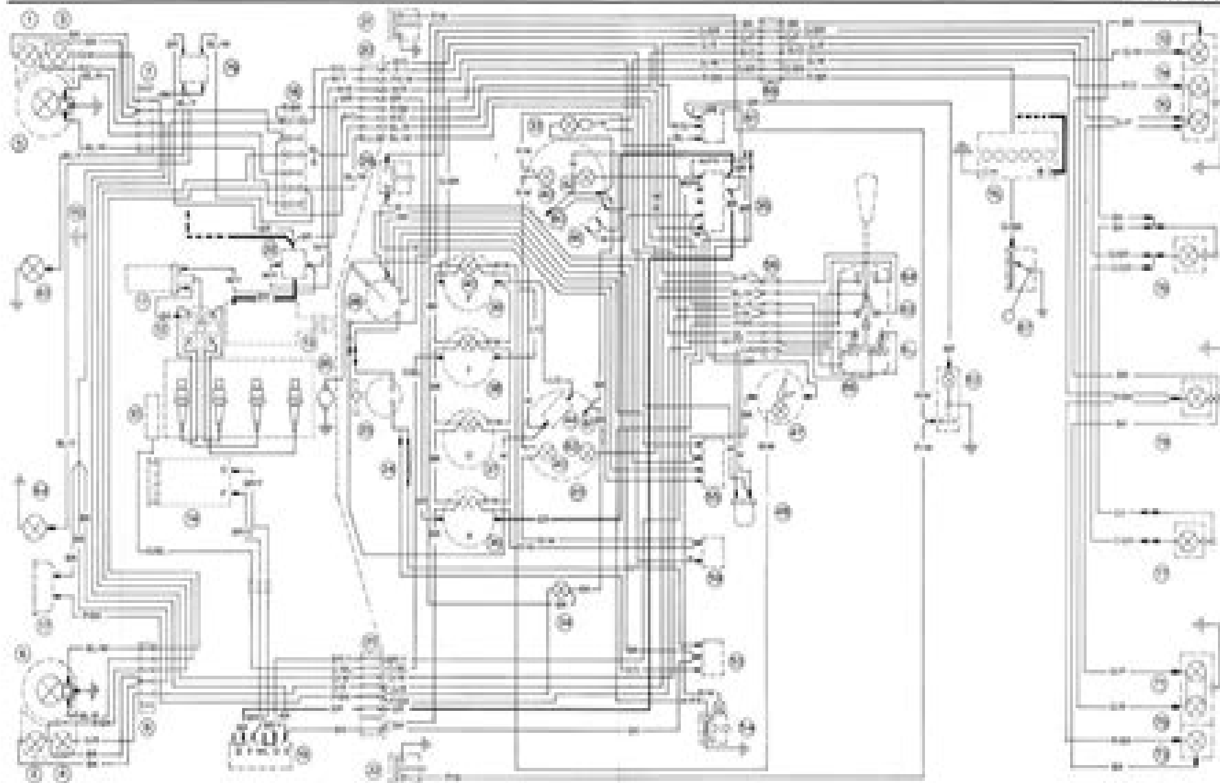
WIRING DIAGRAM - C.A.D. 1980
