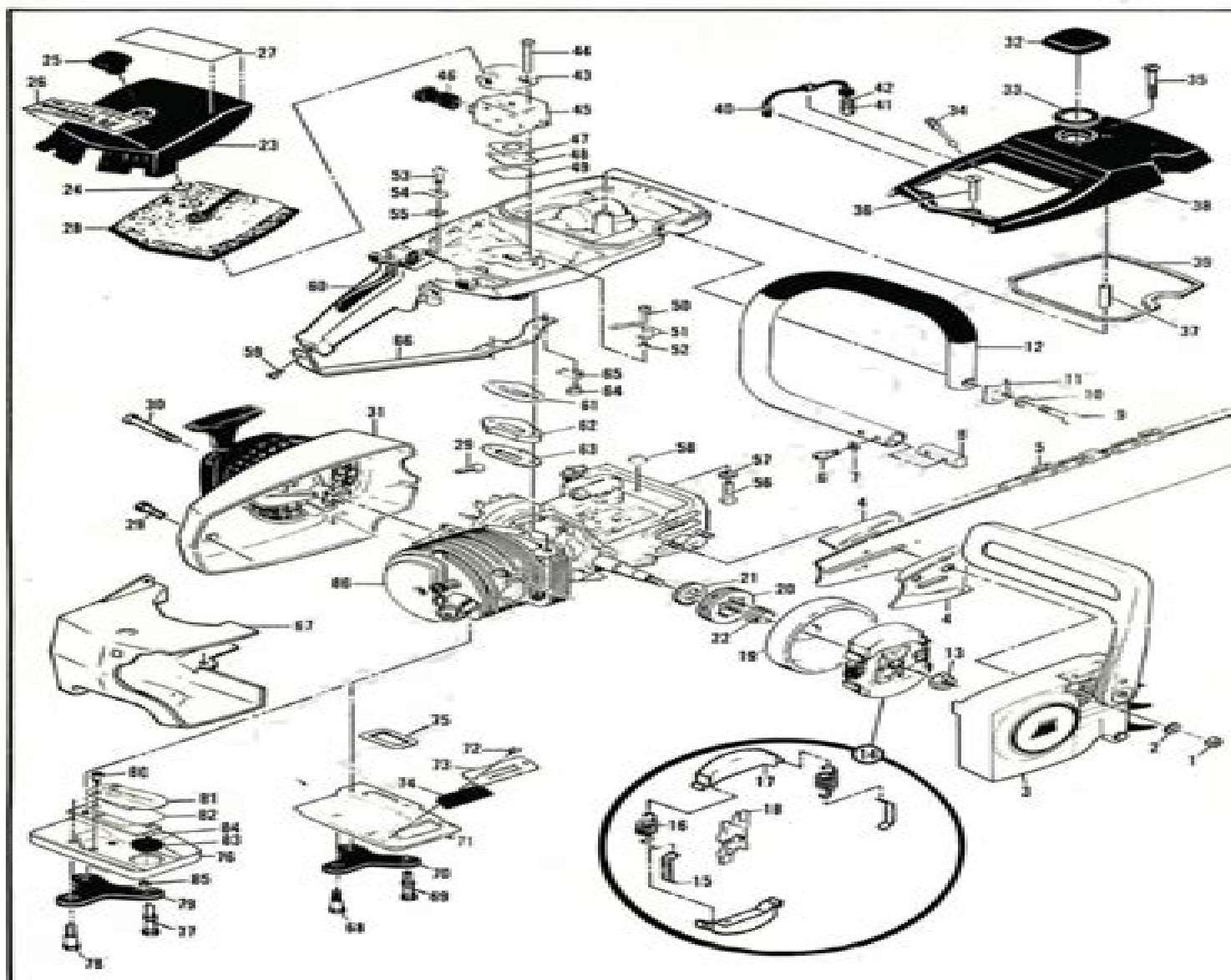
Figure 1. General View - Exploded
