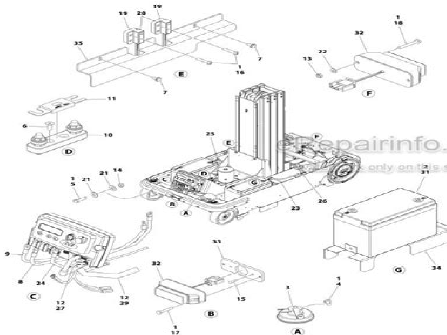
FIGURE 2-2. BATTERIES, ALARM AND STROBE INSTALLATION
