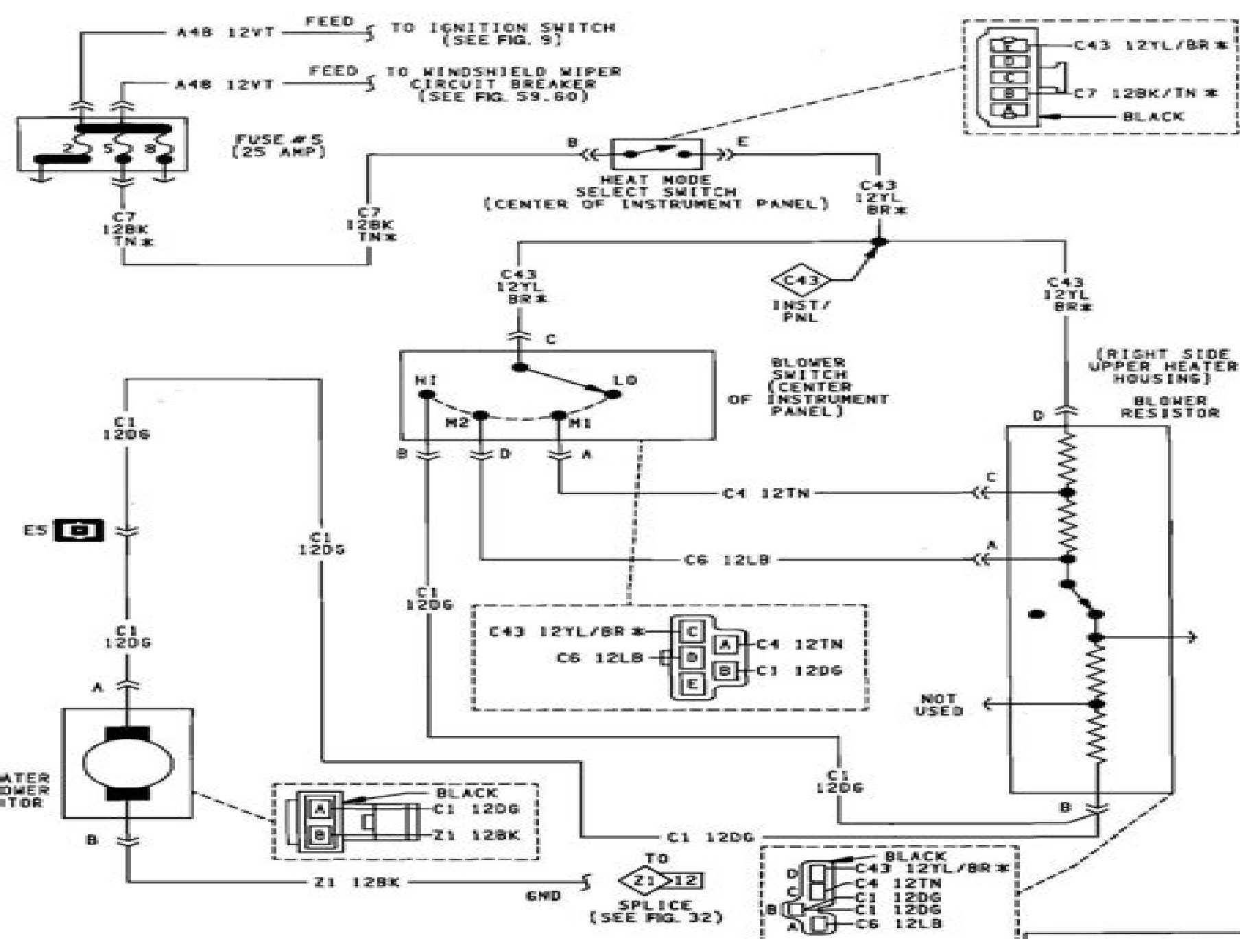
Heater System
