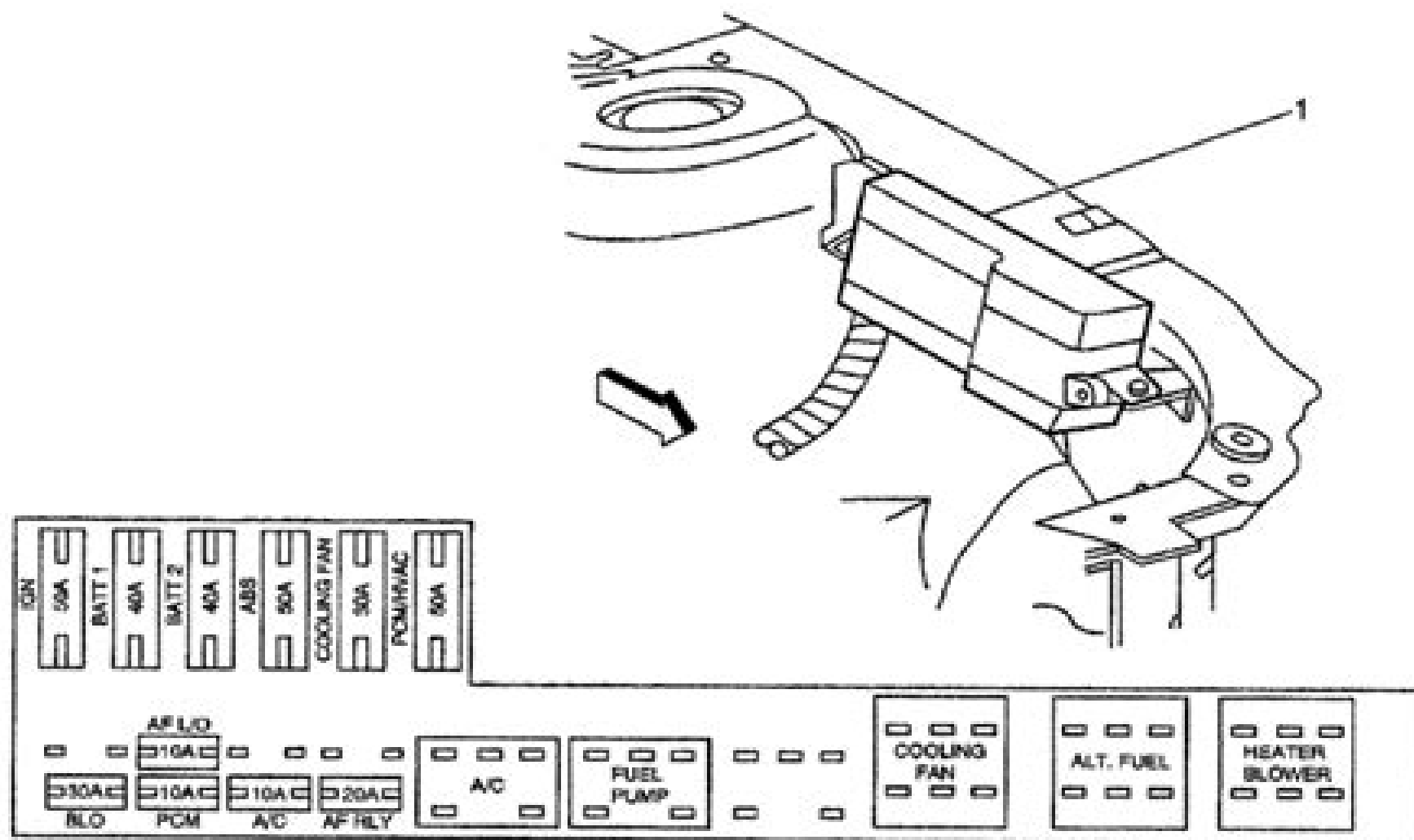
Fig 6: Left Side Of Engine Compartment (CNG)
