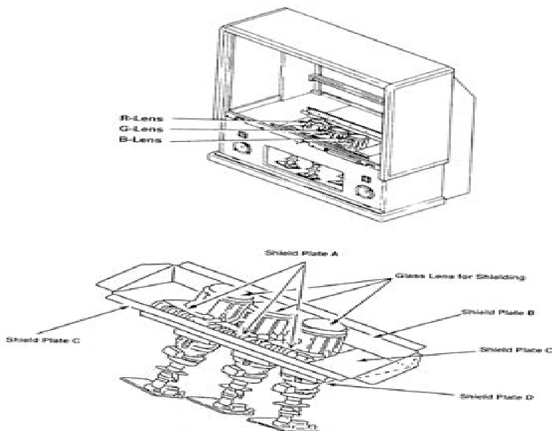
Detailing X-radiation shield. Fig. 1
