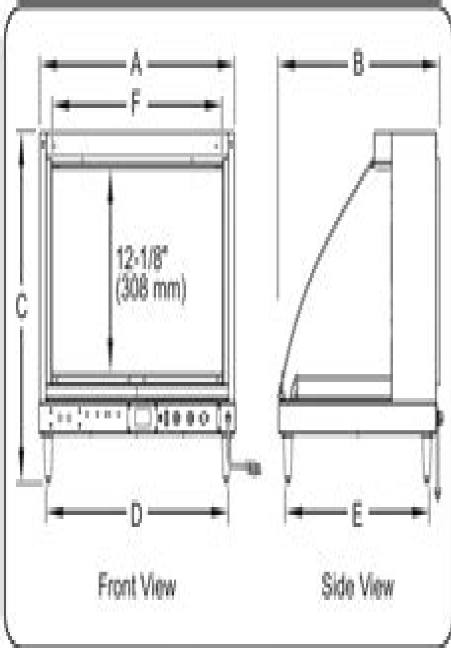
Single Shelf GRCD Dimensions
