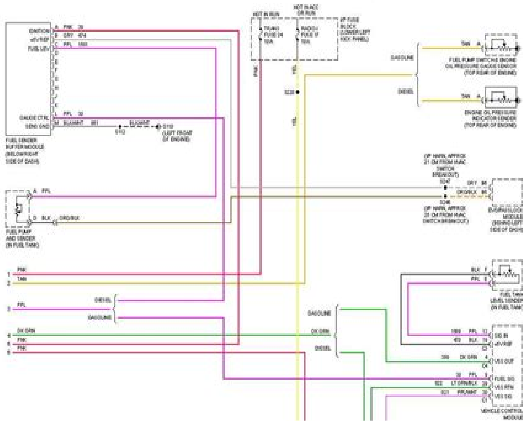
1993 GMC Savana G3500-Fig. 42: Instrument Cluster Circuit (2 of 2)
