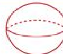
Sphere
