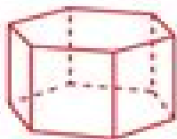
Hexagonal prism
