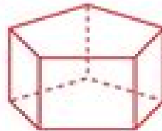
Pentagonal prism
