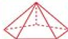
Pentagonal pyramid
