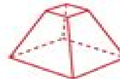
Truncated pyramid
