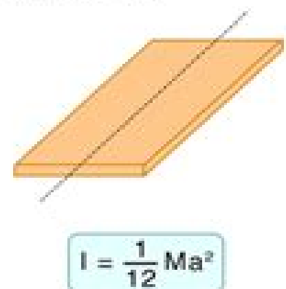
Rectangular plate with axis passing parallelly through the center
