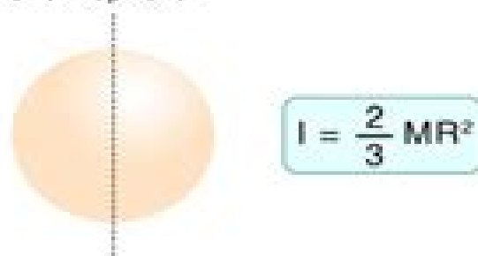
Hollow sphere
