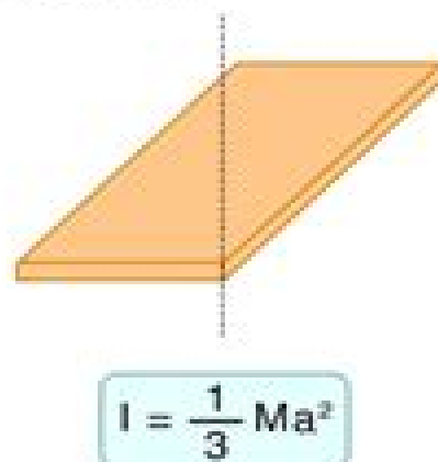
Rectangular plate with axis passing perpendicularly through one edge
