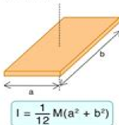
Rectangular plate with axis passing perpendicularly through the center
