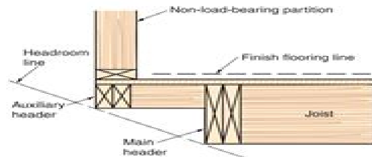
Figure 18-7. Extending the upper floor area with a shallow auxiliary header to provide headroom. The partition over the auxiliary header must not be load bearing.
