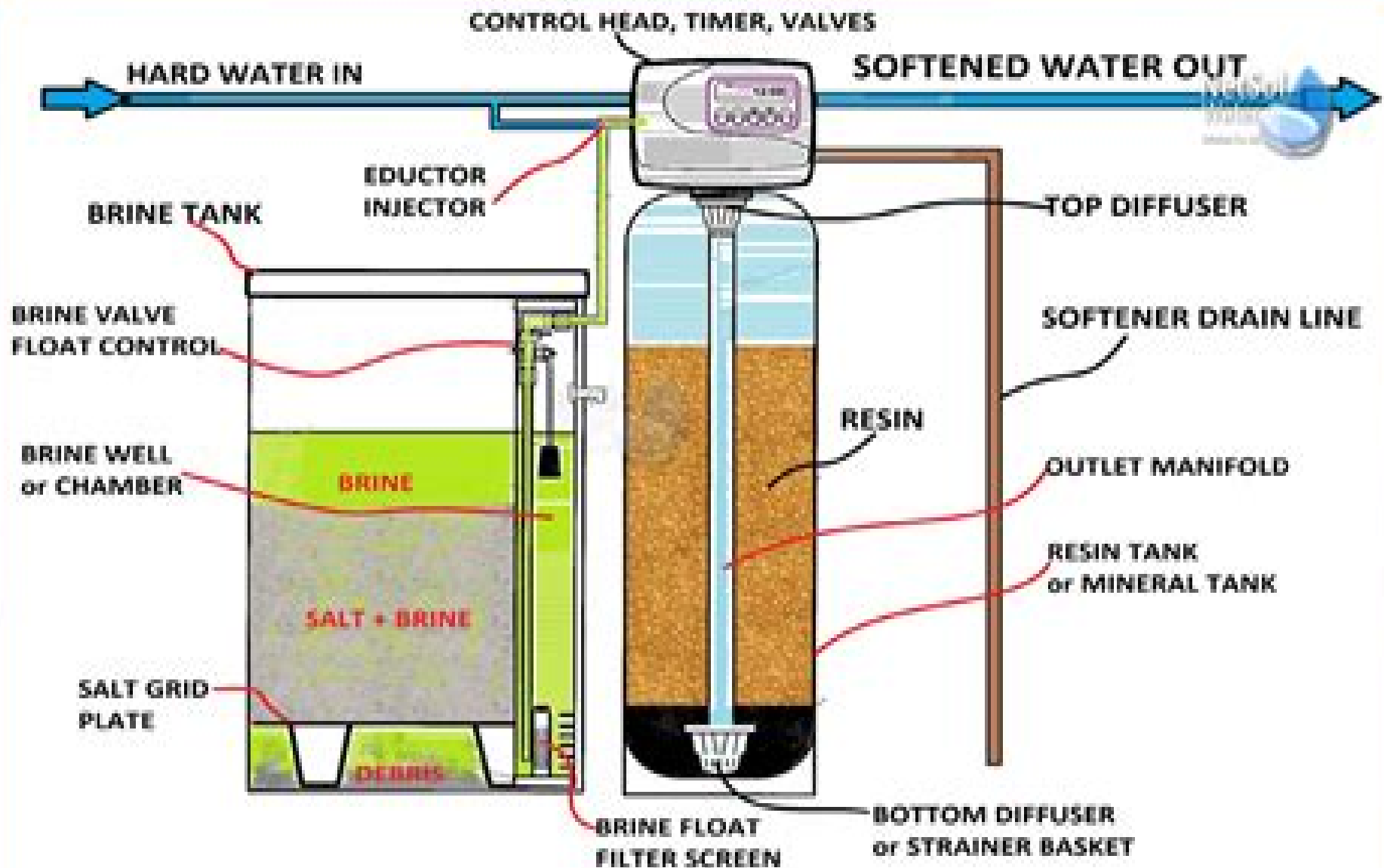
Components of a Water Softener that Comes under O and M Plan
