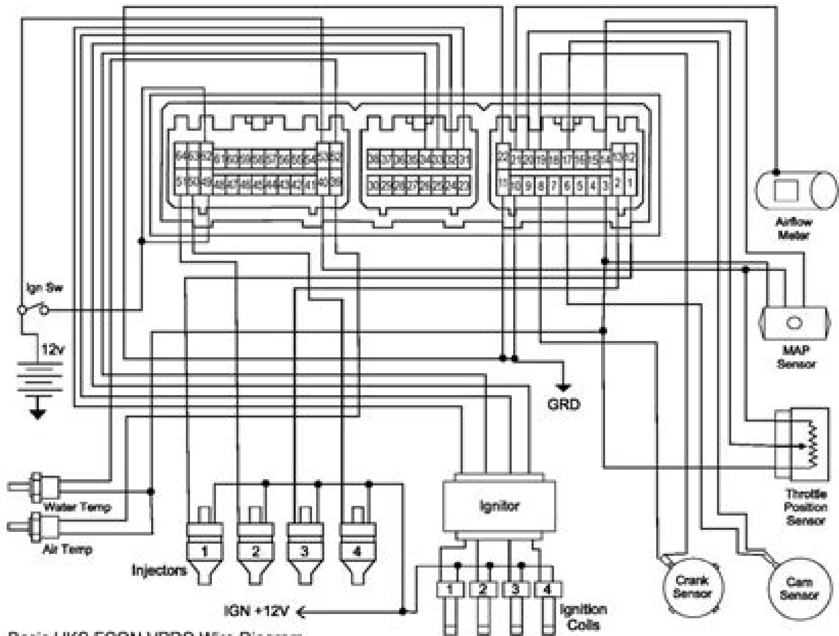
Basic HKS FCON VPRO Wire Diagram
