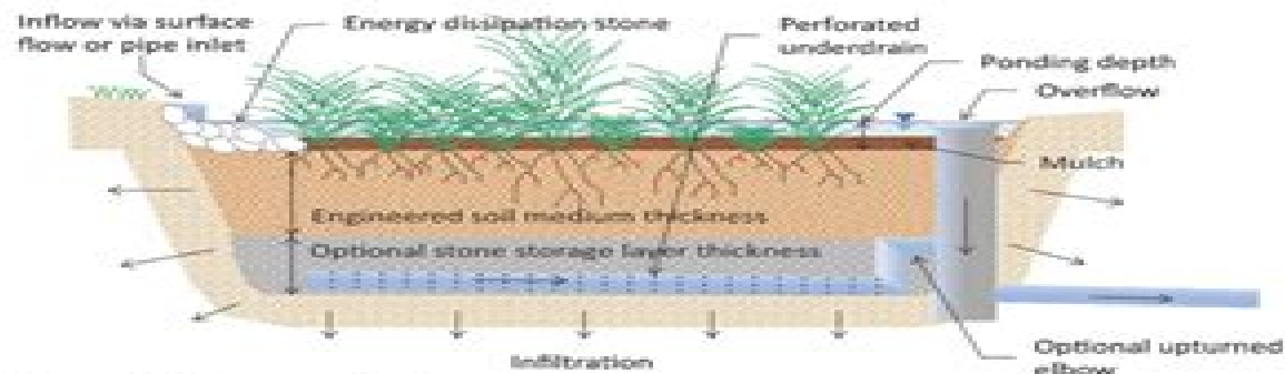
Figure 1. Cross-section view.
