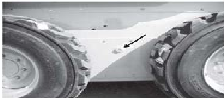
Fig. 3-8 Location of the left chaincase oil fill plug. Right side same.
