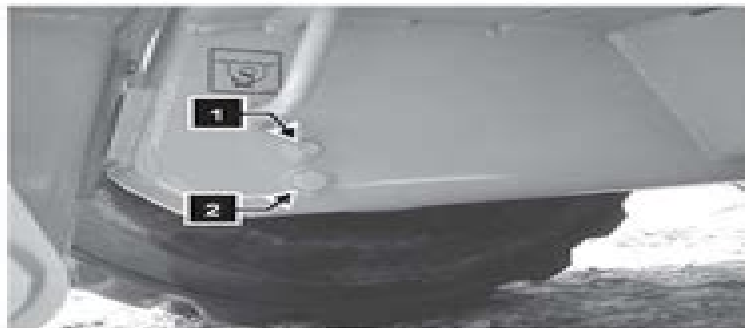
Fig. 3-7 Location of chaincase check plug (1) and drain plug (2) behind right front tire. Left side same.
