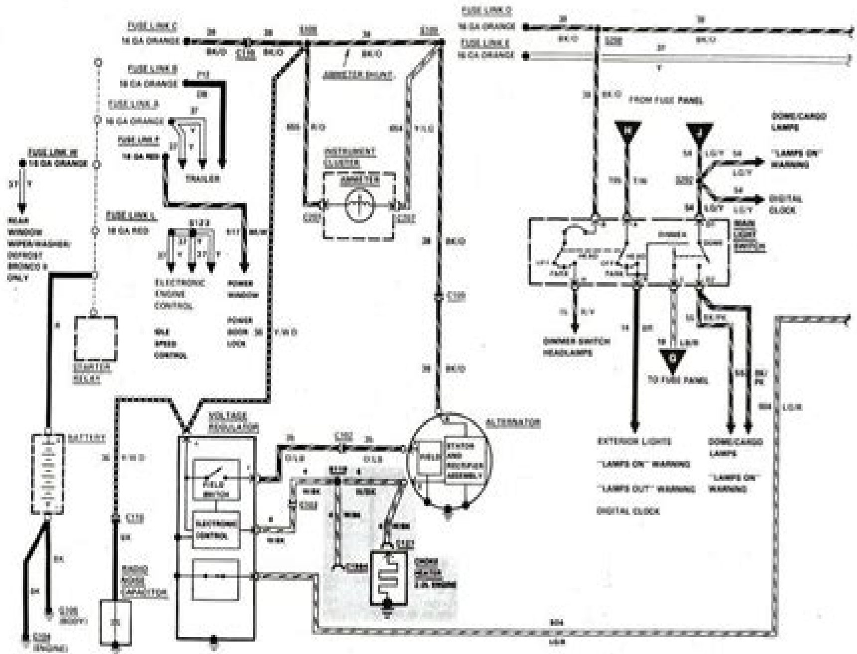
Charging system/power distribution – 1983 through 1985 (part 1 of 2) (ammeter type shown – warning indicator light type similar)
