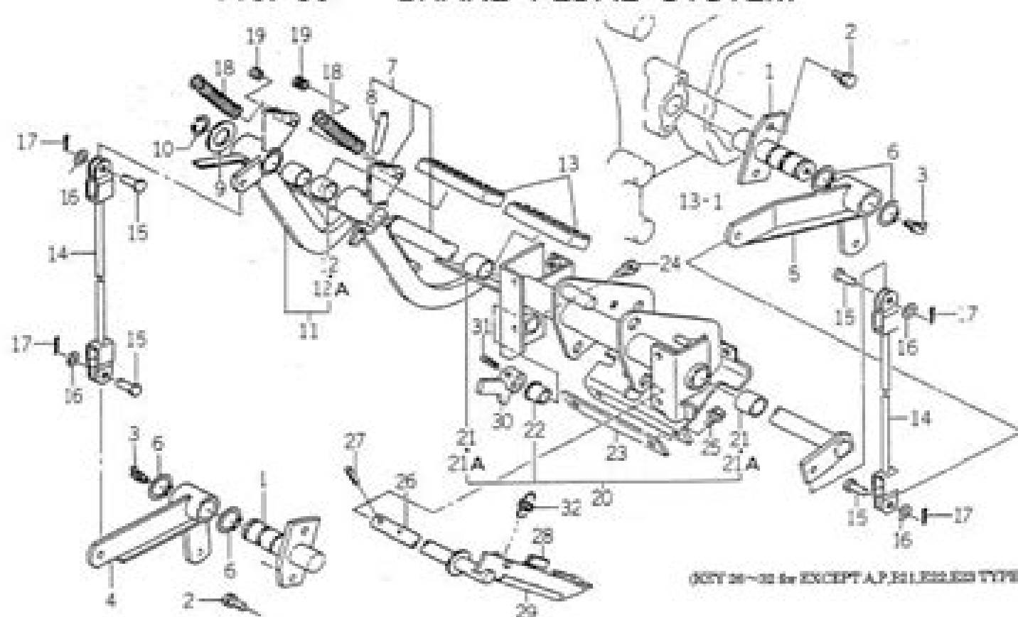
FIG. 35 BRAKE PEDAL SYSTEM
