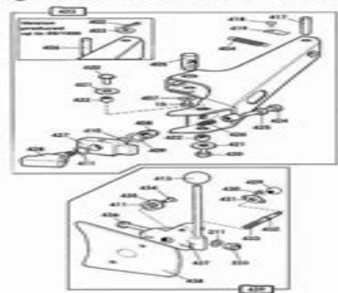
Figure 5B Bead Breaker Arm 3200 PRO
