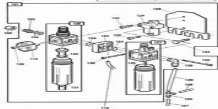
Figure 4 Bead Breaker
