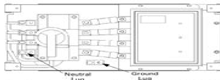
Figure 2. Locations of the ground and neutral lugs in the TVSS unit.
