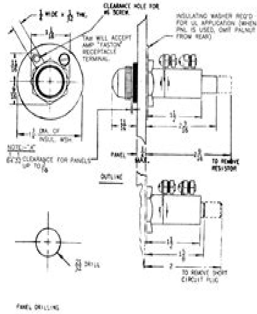
Figure 4. INSTALLMENT, OUTLINE, AND PANEL DRILLING FOR REAR INDICATING LAMP TYPE ET-12
