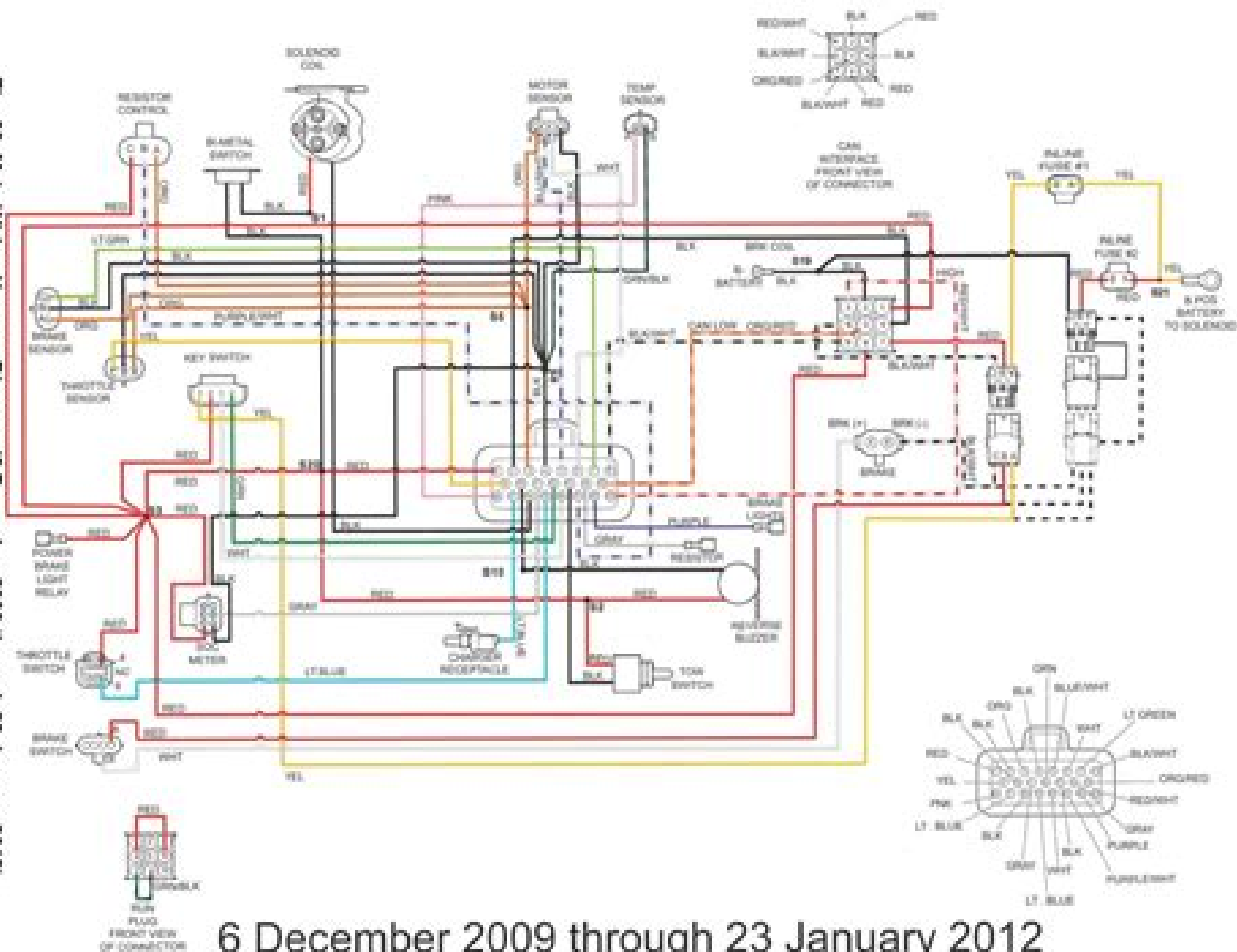
Fig. 30 Main Wiring Harness Diagram (6 December 2009 through 23 January 2012)
