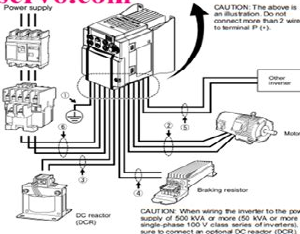
Figure 2.4 Wiring Procedure for Peripheral Equipment
