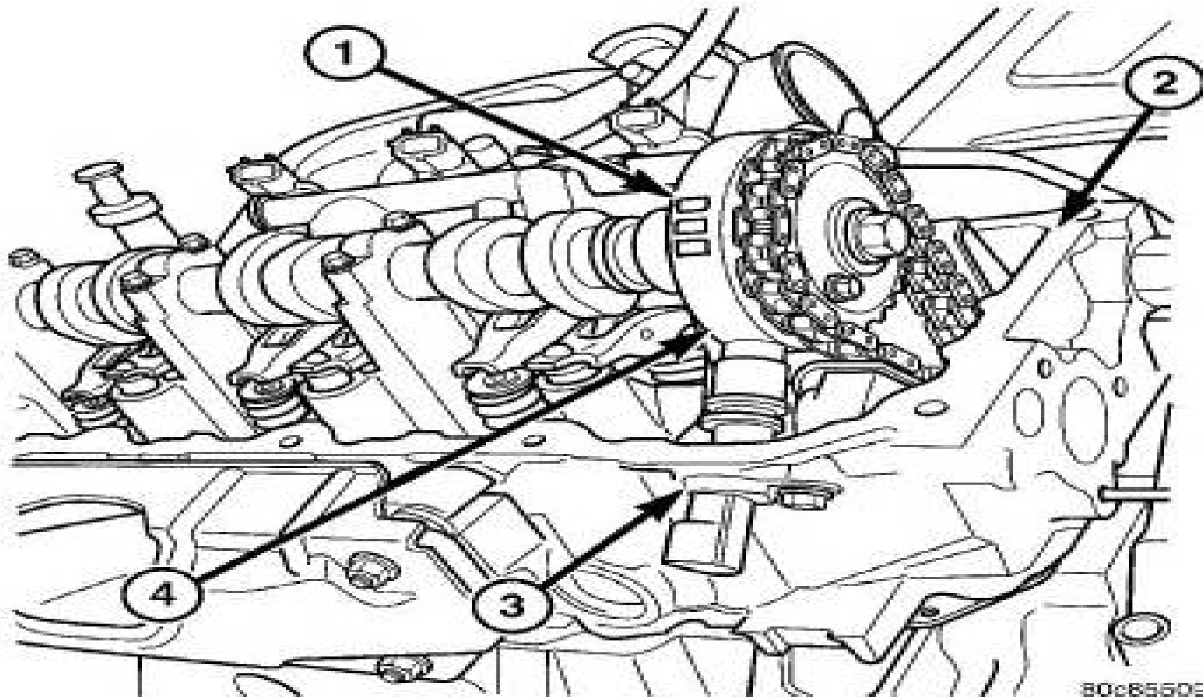
Fig. 8 CAMSHAFT POSITION SENSOR LOCATION
