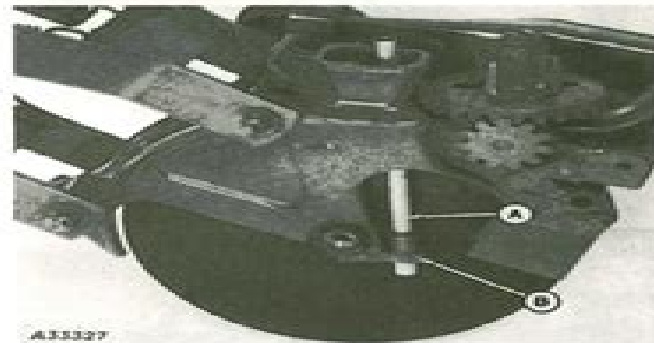
Beet Seed Tube Used with Runner Seed Opener
