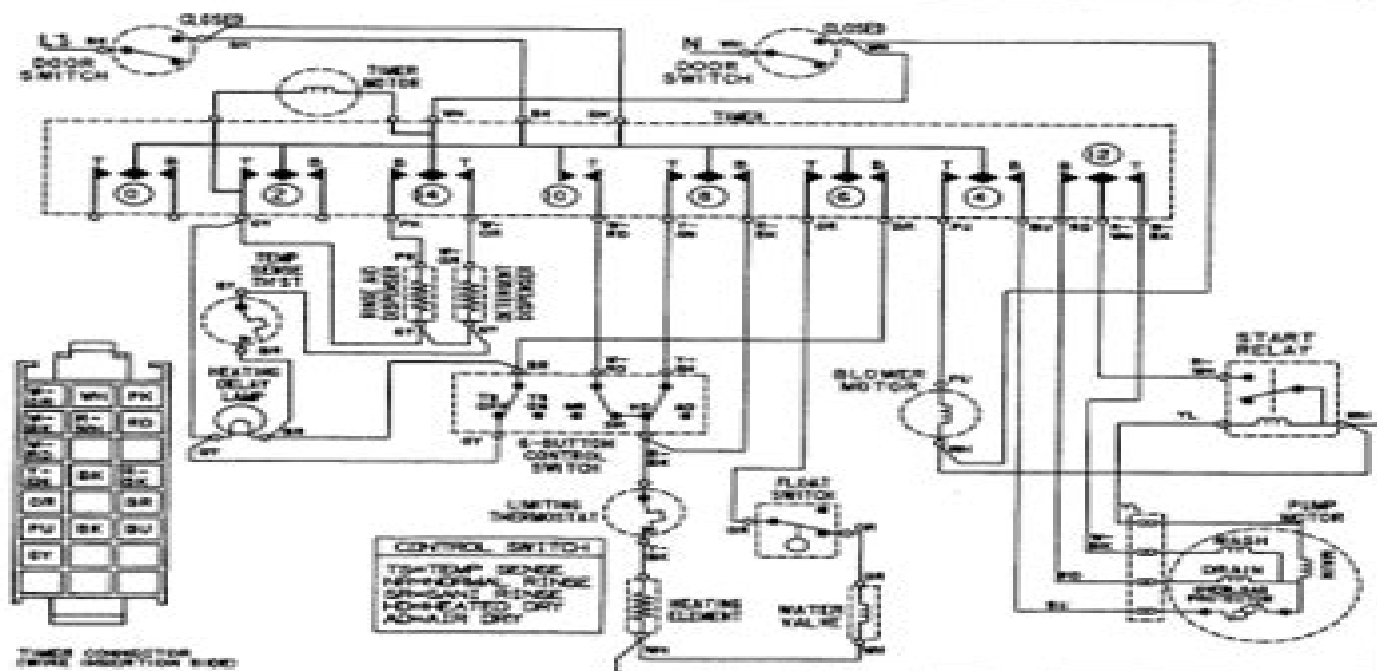
ELECTRICAL SCHEMATIC
