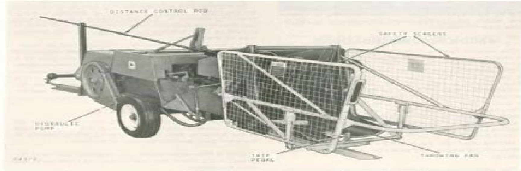
John Deere 30 Bale Ejector on 326 Tractor
