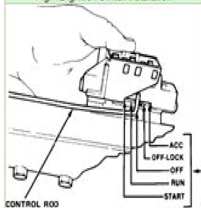
Fig. 12 Ignition Switch Installation
