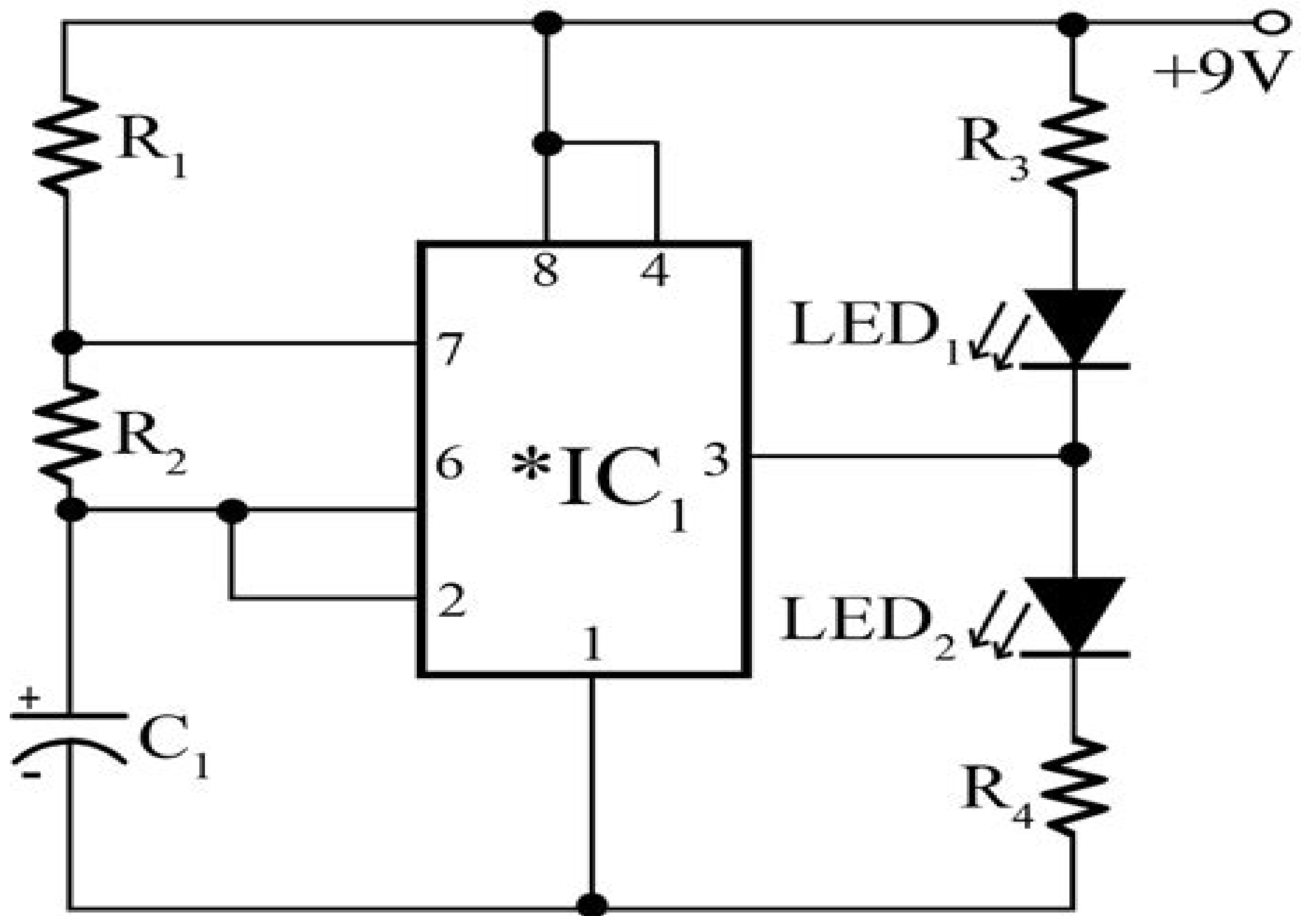
Figure 1: Timer IC (555) Tester
