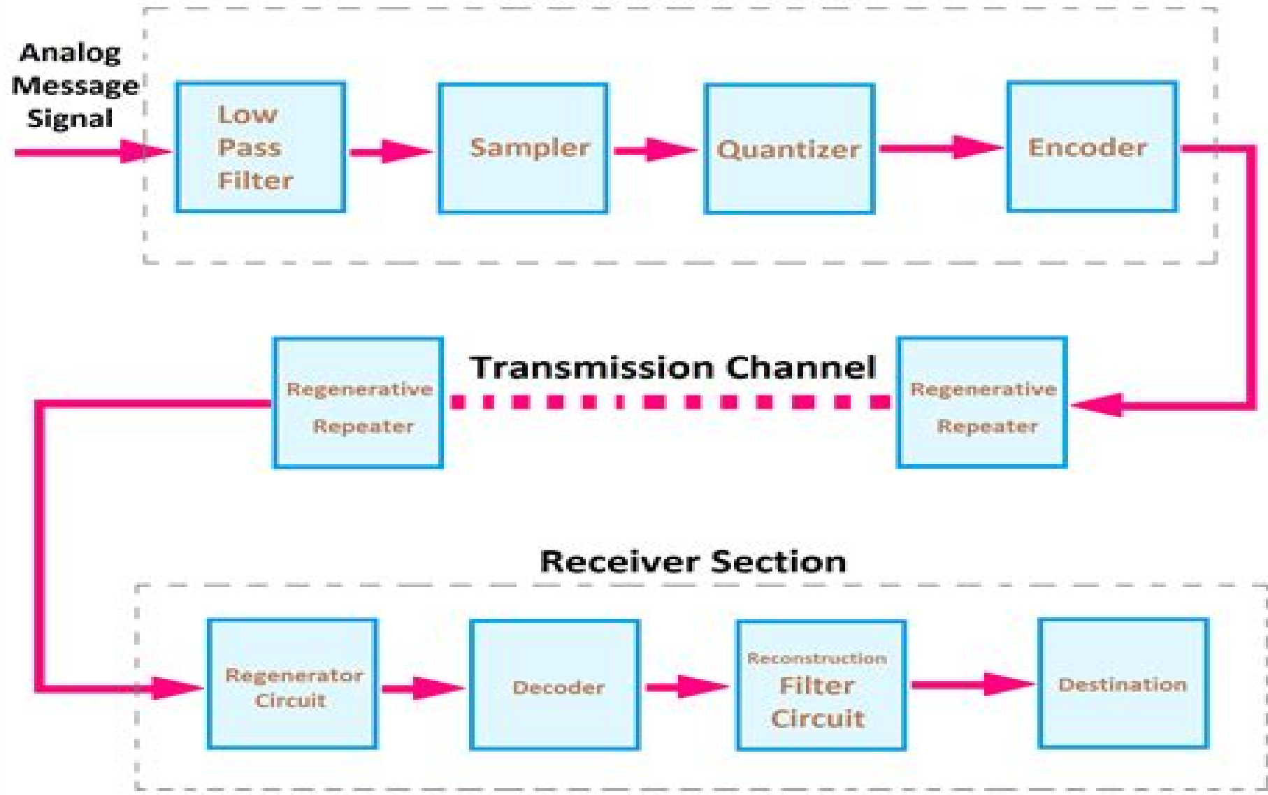
Block Diagram of PCM System
