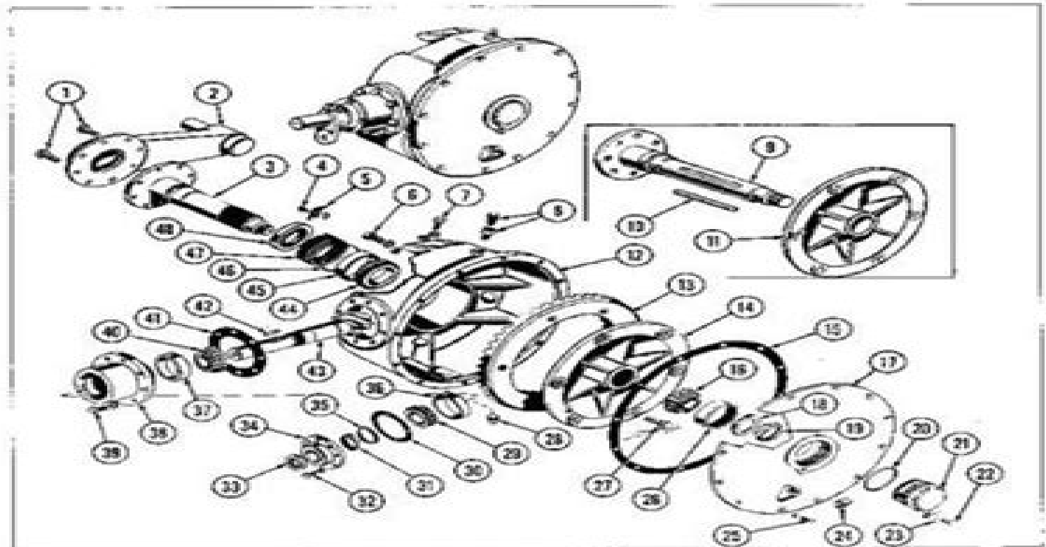
Fig. 1 — Barrel Case Make Drive Assembly
