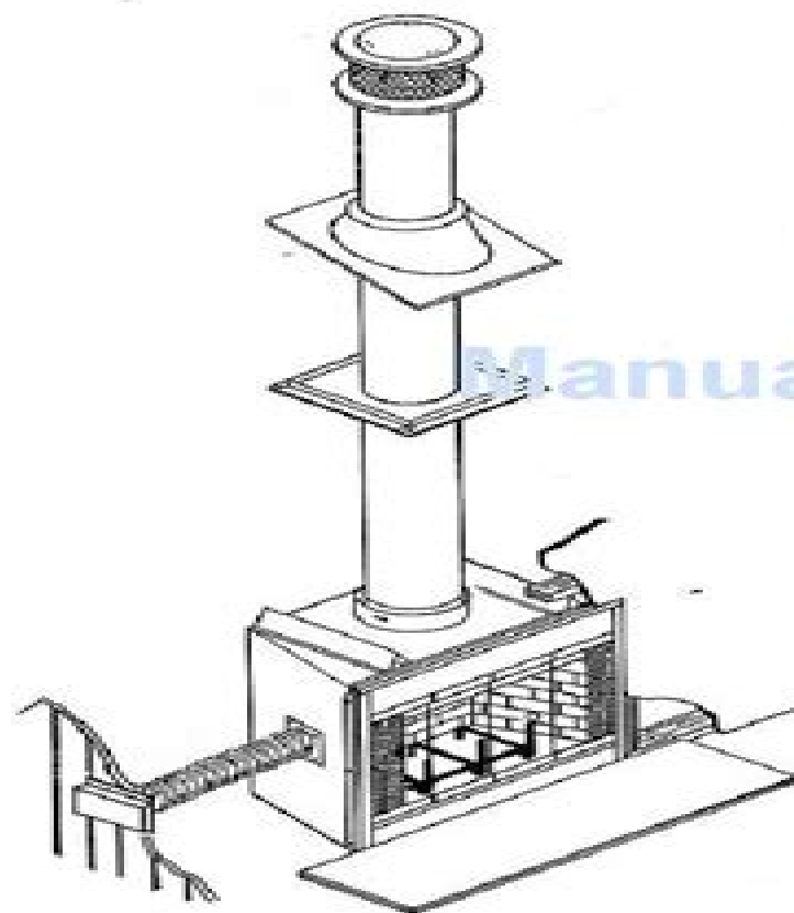
36 INCH BUILT-IN WOOD BURNING FIREPLACE WITH OPTIONAL OUT- SIDE AIR FOR COMBUSTION, GLASS DOORS, AND FAN ASSEMBLY
