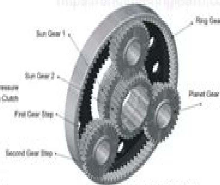
Planetary Gearbox
