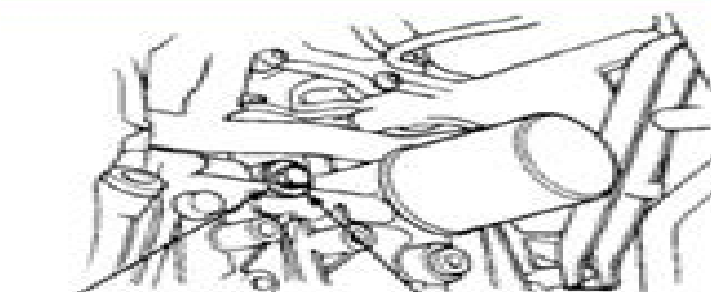
DRAIN BOLT 60 N·m (6.0 kg-m, 43 lb-ft) Apply liquid gasket to the bolt threads when installing.
