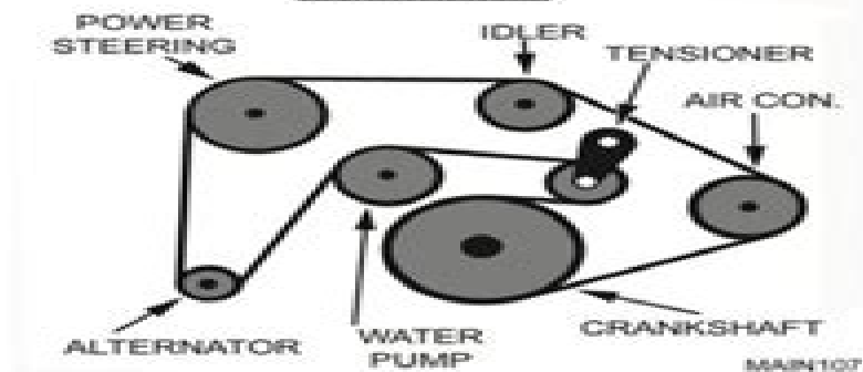
6 Cylinder Drive Belt
