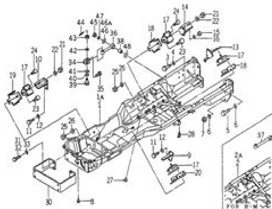
FIG. 51 FRAME SYSTEM
