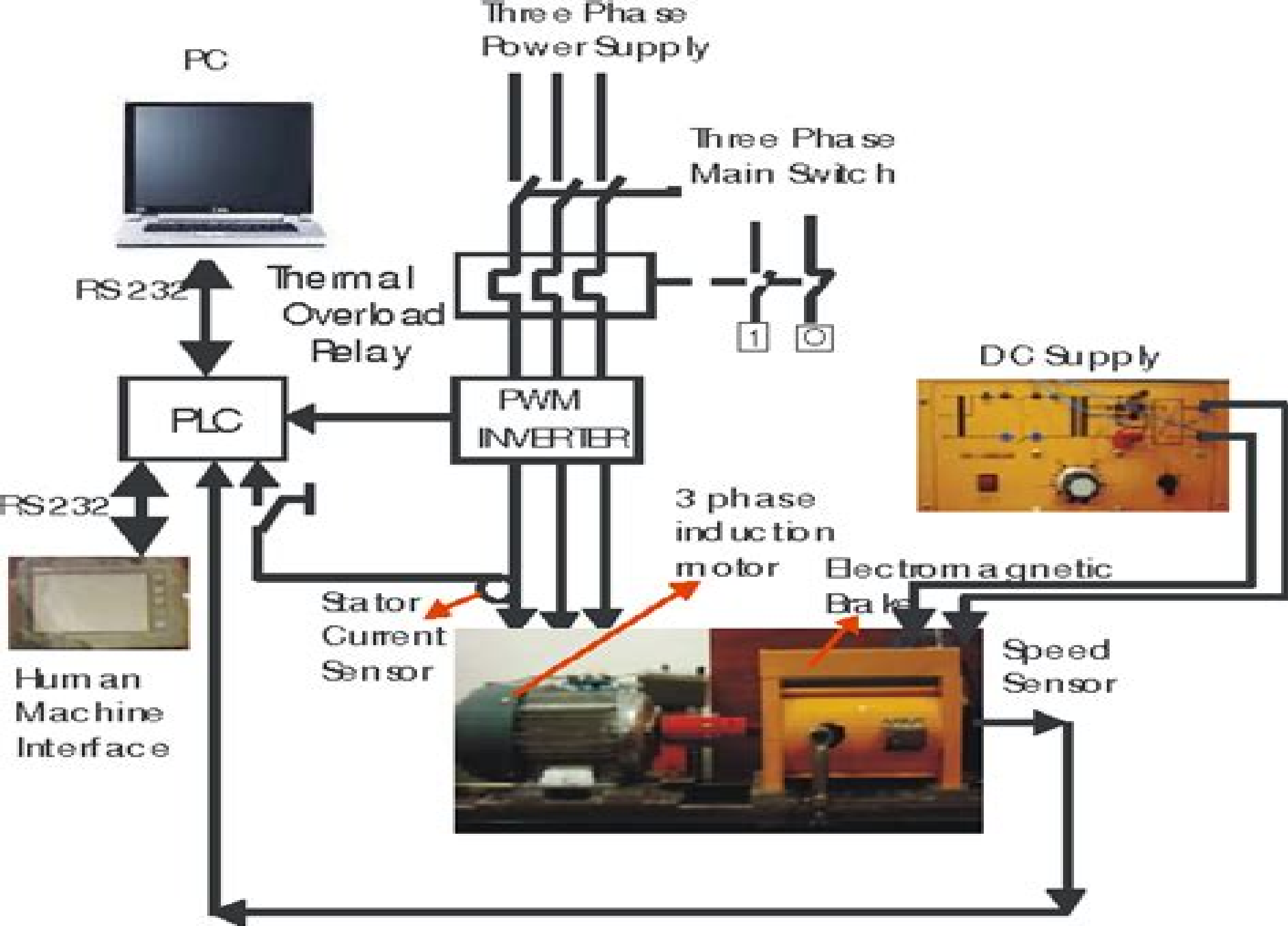
Fig. 2. Experimental setup
