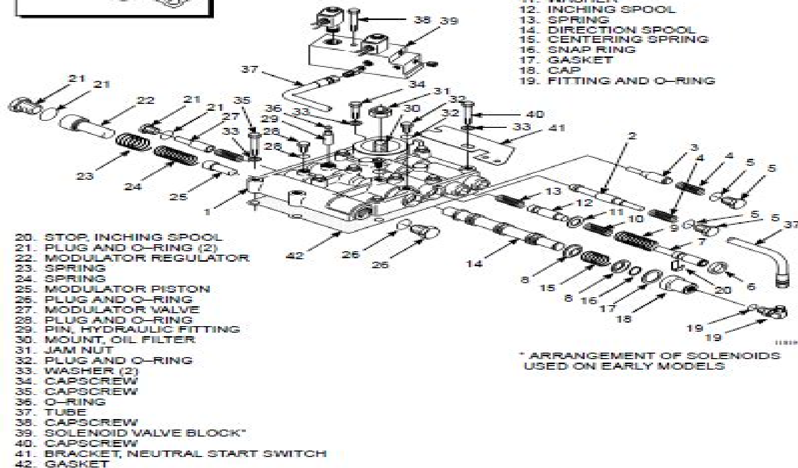
FIGURE 10. CONTROL VALVE, MONOTROL ONLY
