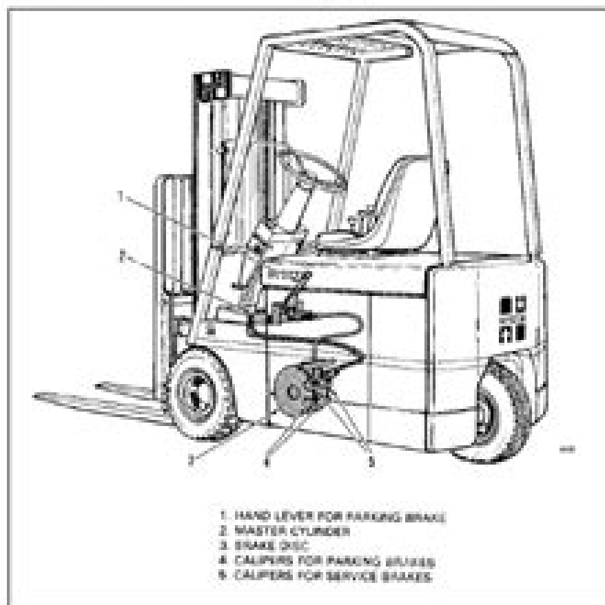
FIGURE 1. LOCATION OF BRAKE SYSTEM COMPONENTS
