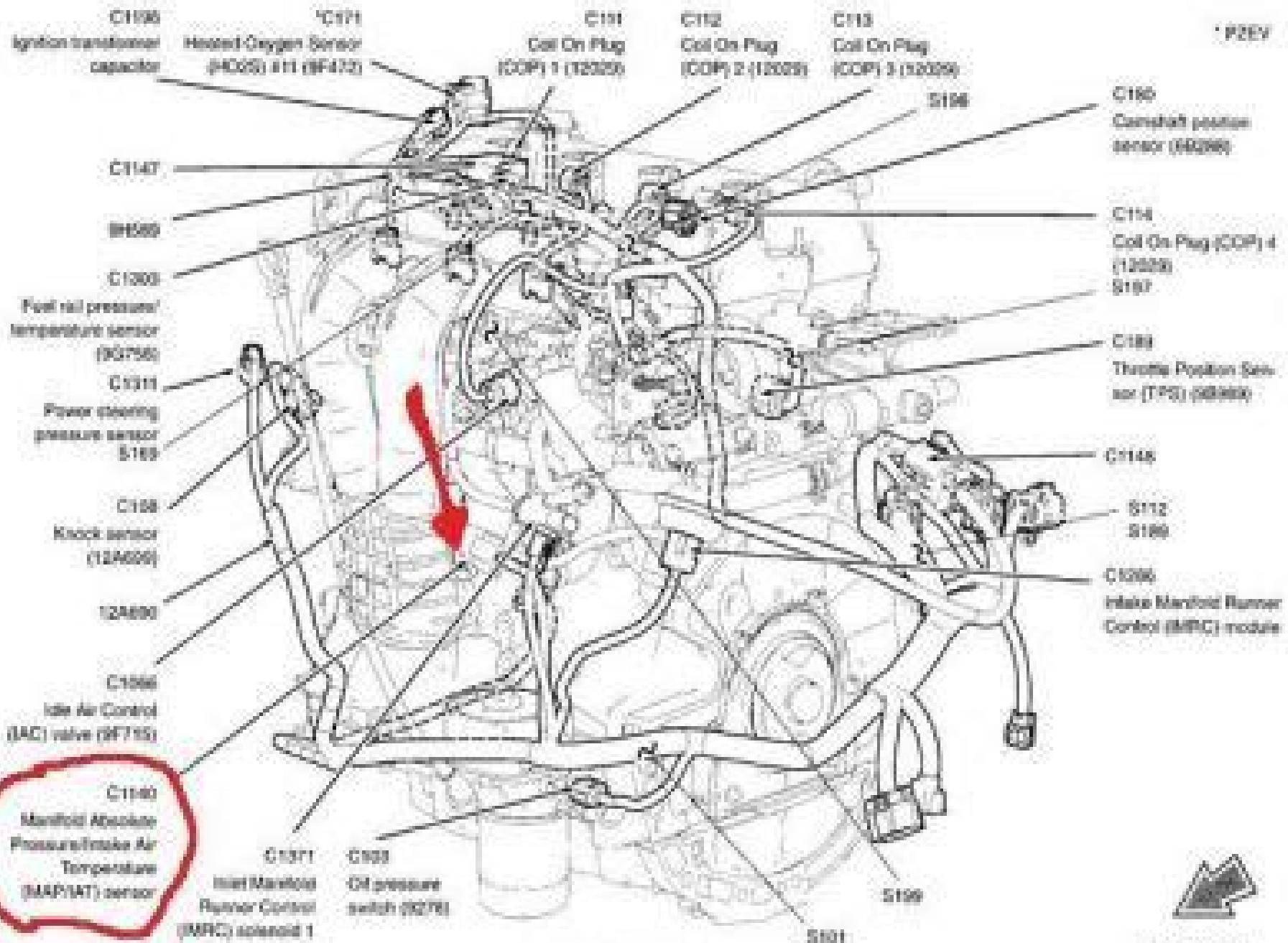
engine, front - 2.0L
