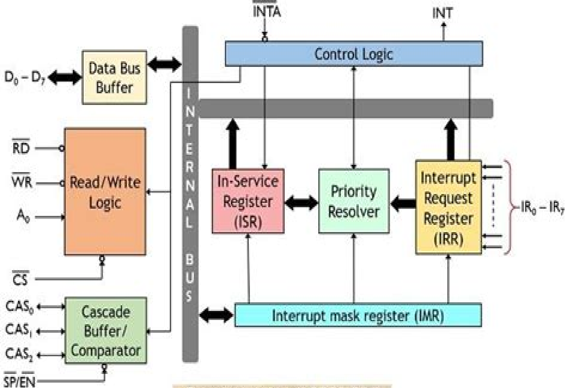
Architecture of 8259 PIC
